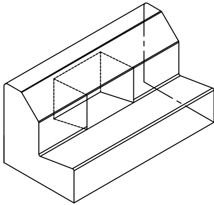
ISOMETRIK
