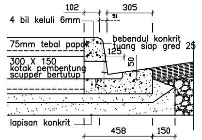
(KERATAN TIPIKAL LUBANG SCUPPER)
