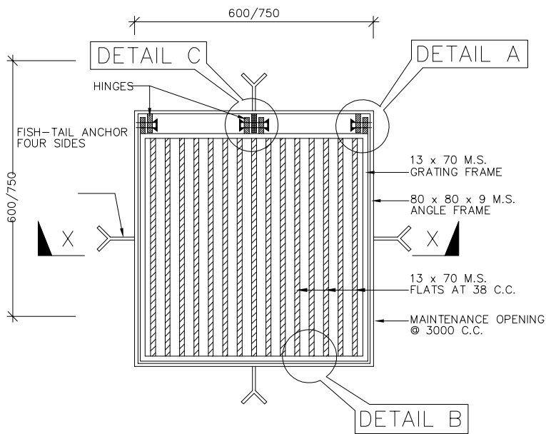
TYPICAL PLAN OF PROP. HEAVY DUTY M.S. GRATING 600/750 WIDTH NOT TO SCALE
